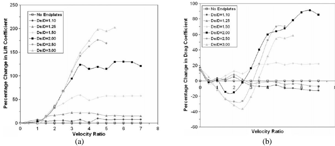
Figure 2 Effect of De/D_0 on Lift (a) and Drag (b) Coefficients [8]
