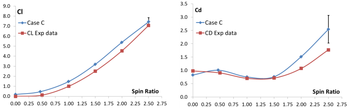
Figure 6 Comparison between experimental data and numerical results with grid uncertainty
