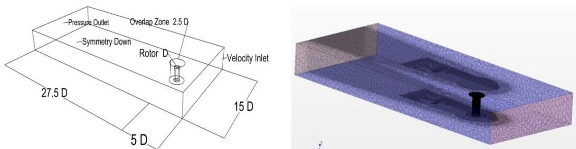
Figure 4 Simulation domain with boundary conditions (a) and mesh visualization (b)
