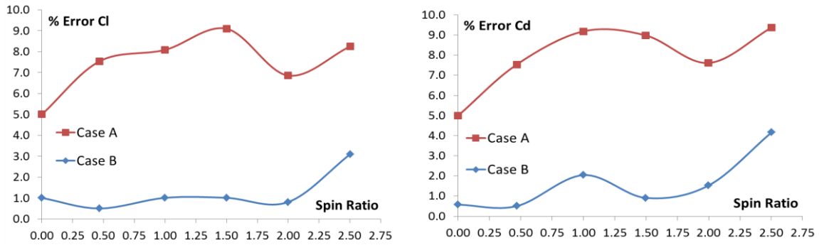
Figure 5 C_1 and C_d percentual error of finer grid (Case C)
